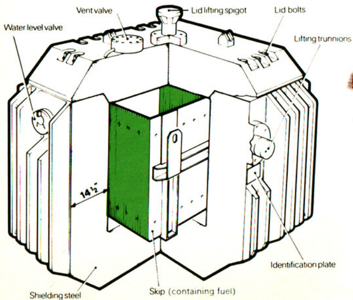
Magnox irradiated fuel transport flask.
