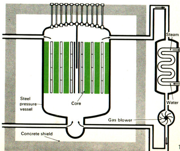
Magnox Reactor.
