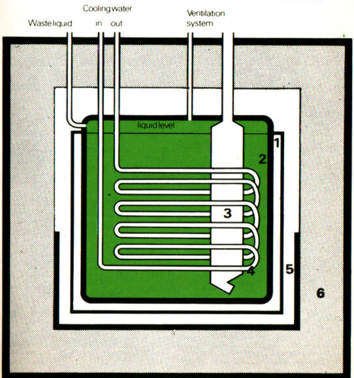
Fission product storage tank.
