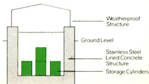
Fission product glass storage.
