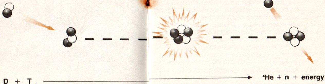
The Deuterium-Tritium Fusion Reaction.
