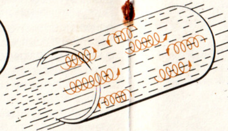
Charges in a magnetic field
