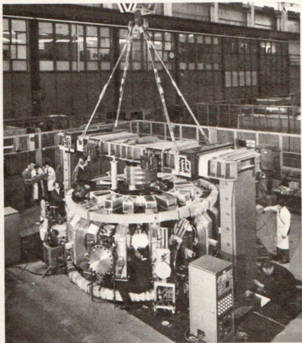
A tokamak under construction.
