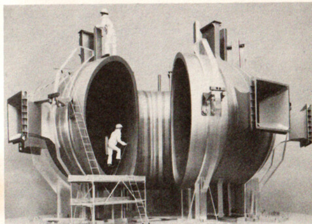
Scale model of the vacuum chamber of the JET fusion experiment.
