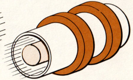
Plasma in a magnetic field
