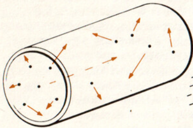
Without magnetic field
